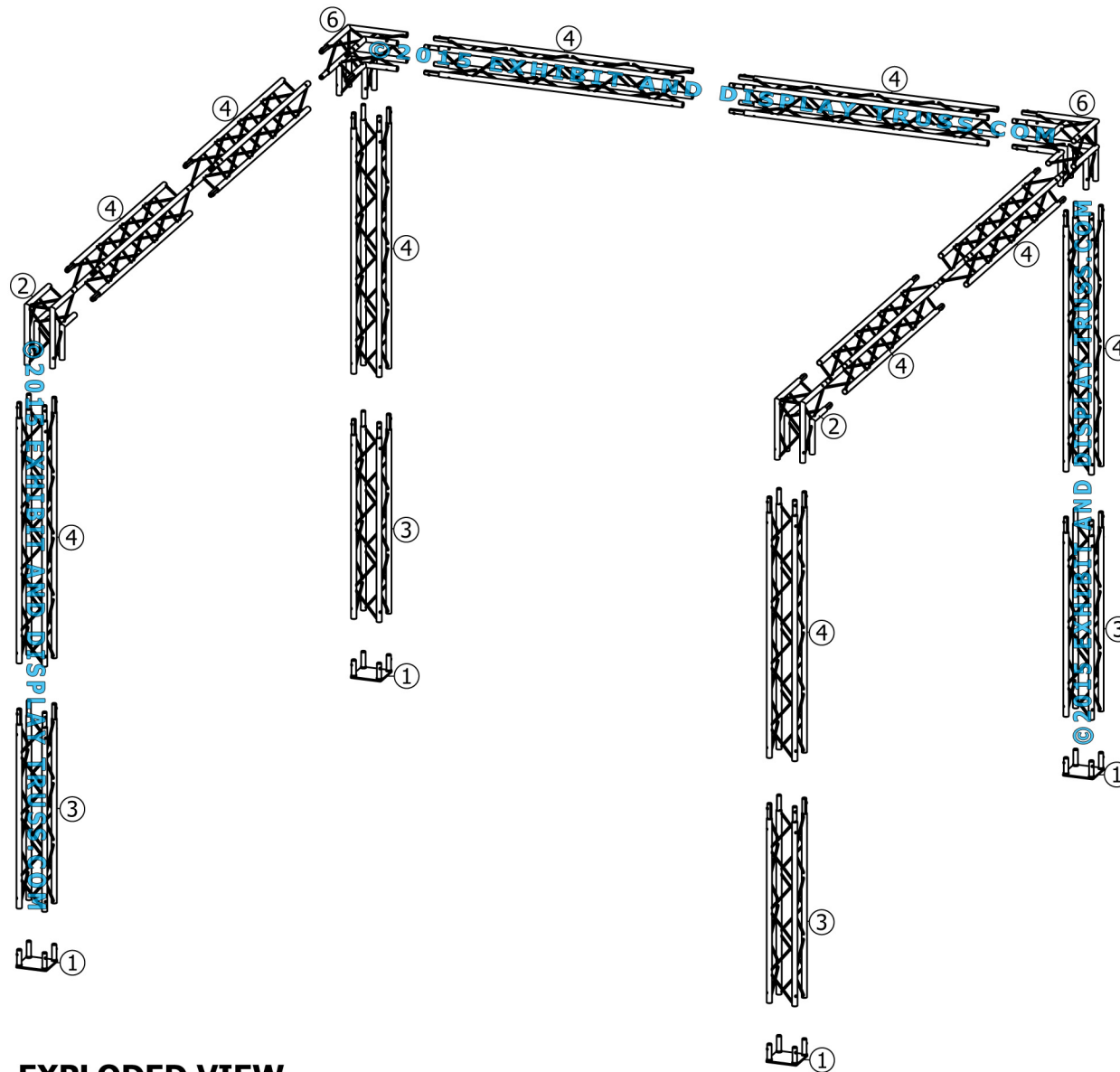
EXPLODED VIEW
